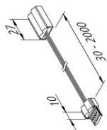
connecting cable LED Twin-Stick 2
