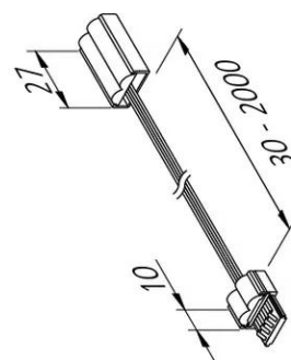
connecting cable LED Twin-Stick 2
