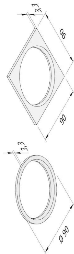
adapter rings
