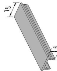
LED Cover Profile 15mm
