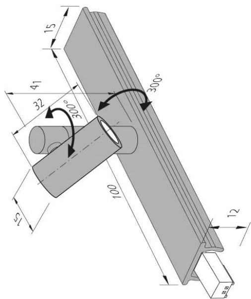
LED 24
